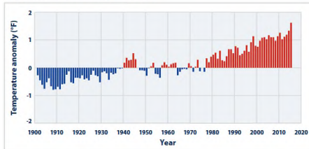
Temperatures Worldwide, 1901-2015
